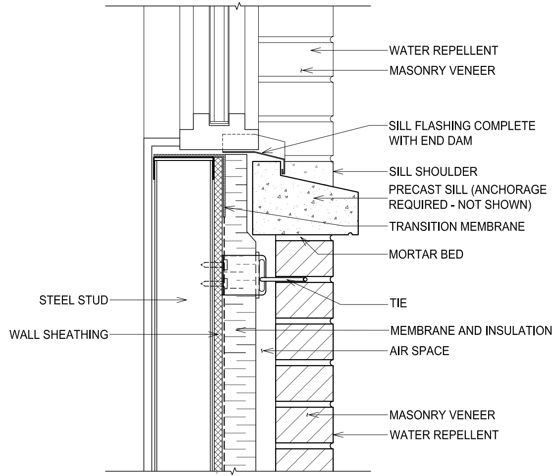
VENEER DETAILS - STEEL STUD AT WINDOW SILL - PRECAST CONCRETE SILL - DETAIL S3.1
