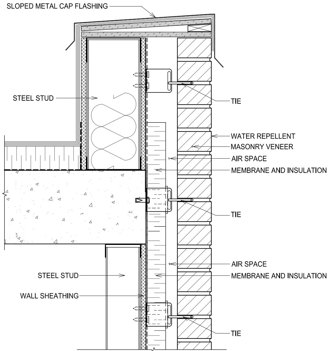
VENEER DETAILS - STEEL STUD BACKUP AT ROOF - LOW PARAPET - DETAIL S6
